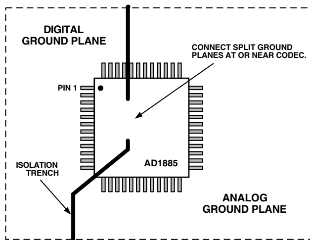
Figure 18. Recommended Split Ground Plane
