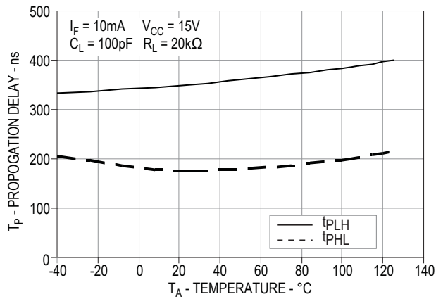
Figure 8. Propagation Delay with External 20 kΩ RL vs. Temperature.
