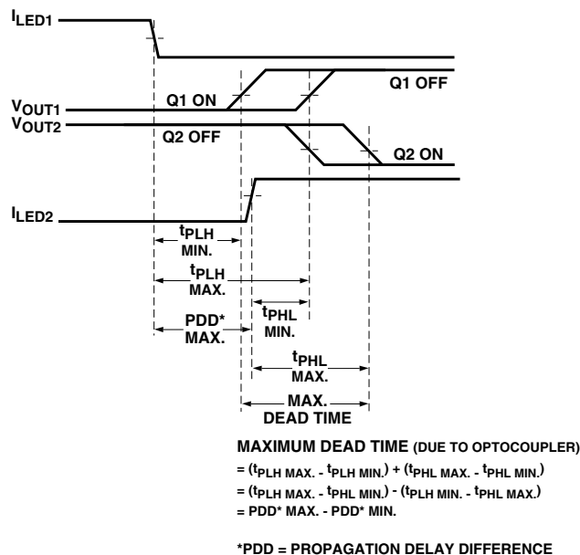
Figure 24. Waveforms for Deadtime Calculation.
