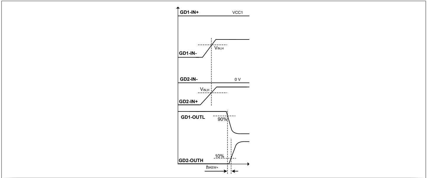
Figure 34 Skew plus using the inverting and non-inverting inputs with rising edges
