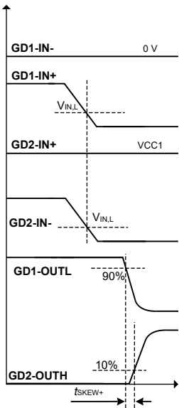
Figure 33 Skew plus using the inverting and non-inverting inputs with falling edges
