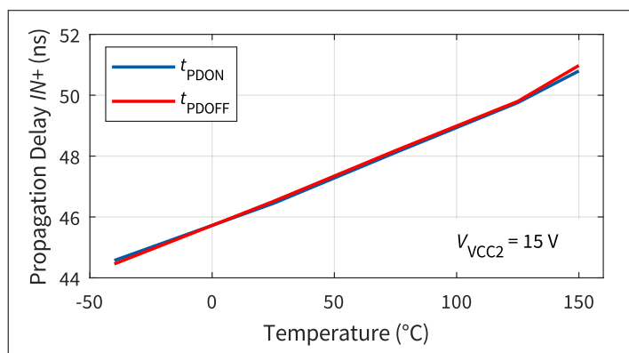
Figure 19 Propagation delay for IN+ vs. temperature ( V_{VCC2} = 15\text{ V} )
