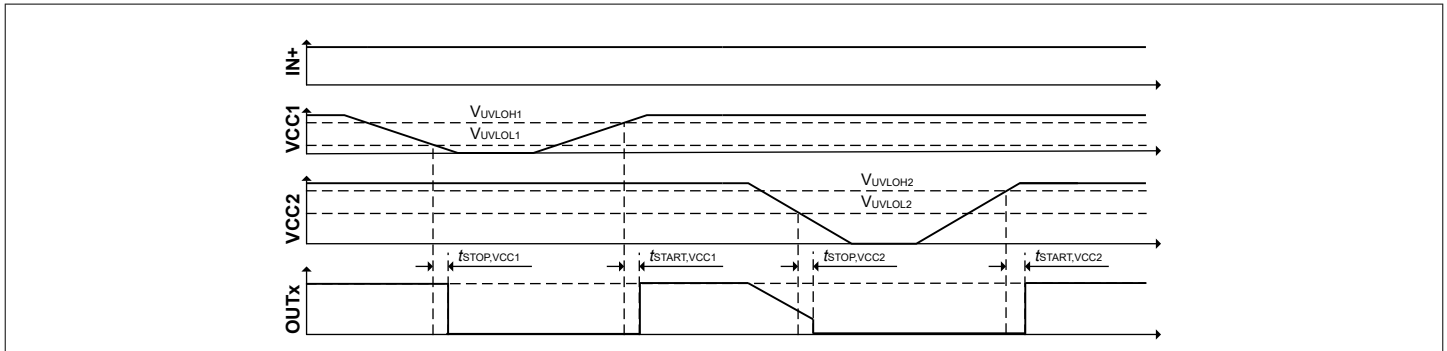
Figure 35 UVLO behavior
