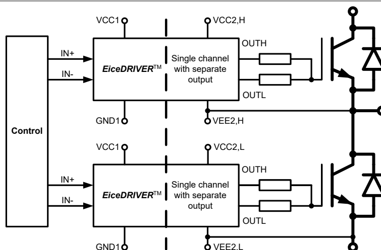
Typical application diagram
